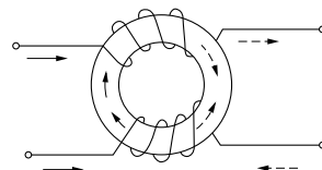
→ Current of Common Mode (Noise) - - - Current of Differential Mode (Signal)
